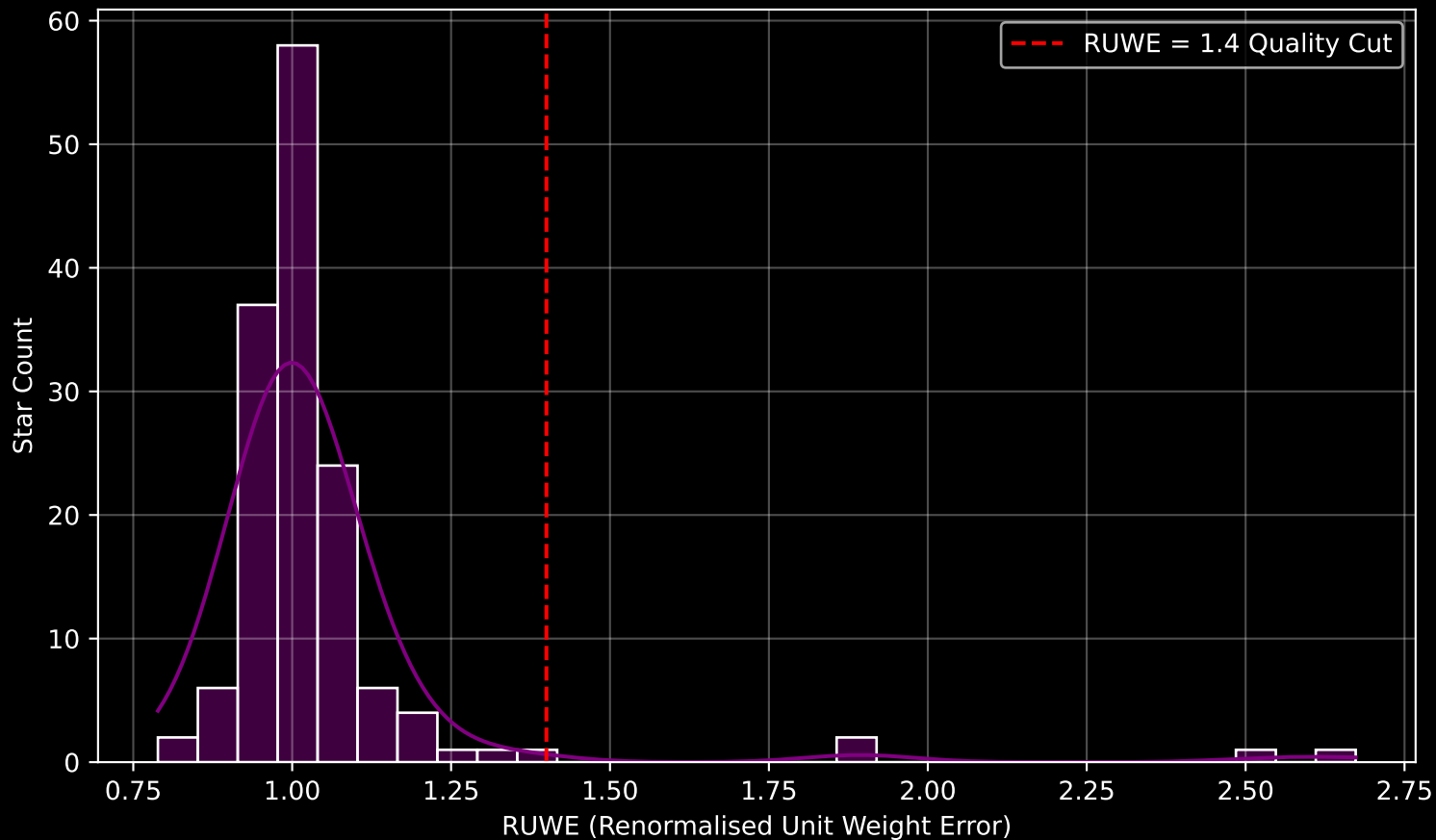
GAPOGEE DR17 Field [SGRC-3] RUWE Distribution (n= 144)
