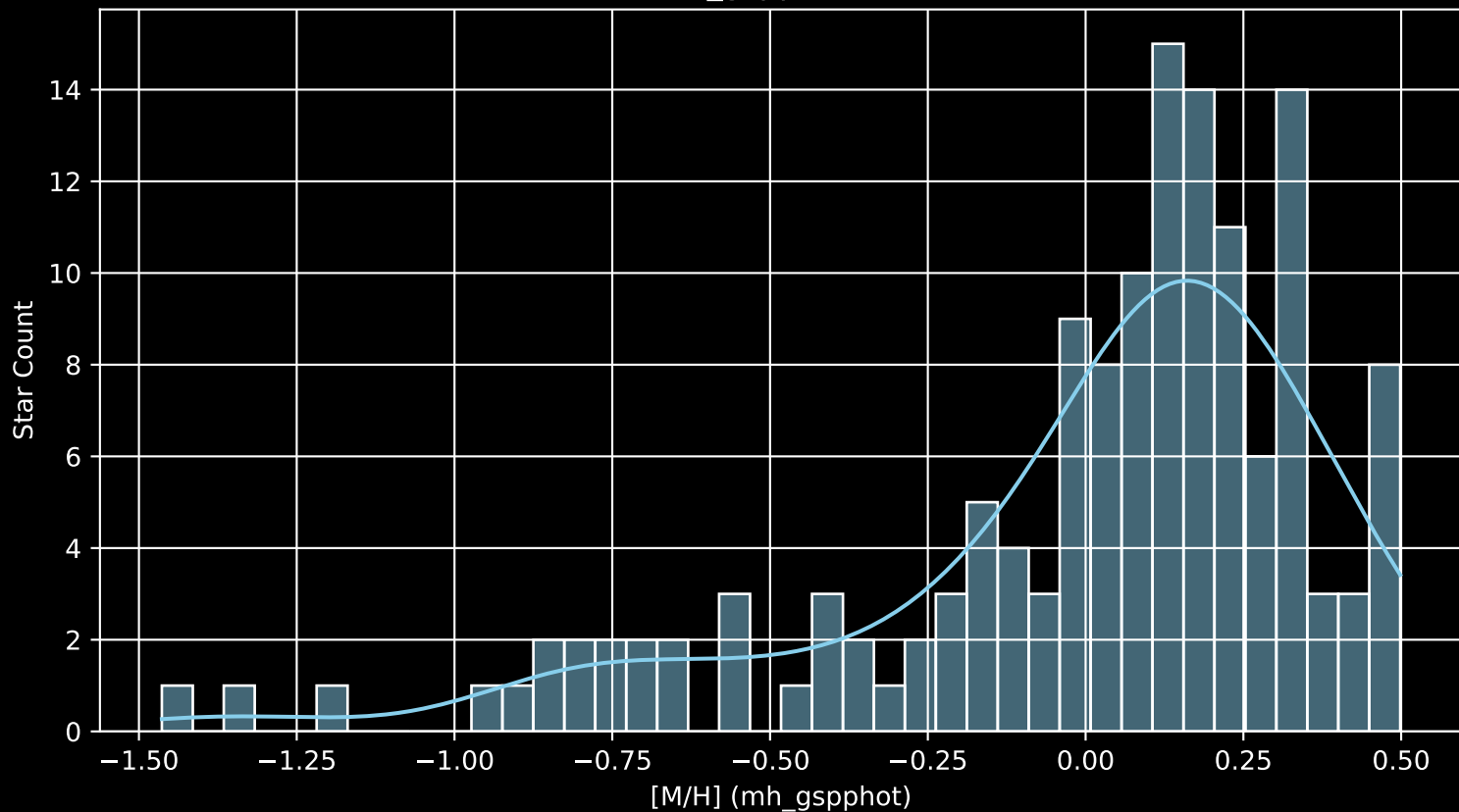
APOGEE DR17 Field: [SGRC-3 [M/H] (mh_gspphot) (n= 143)
