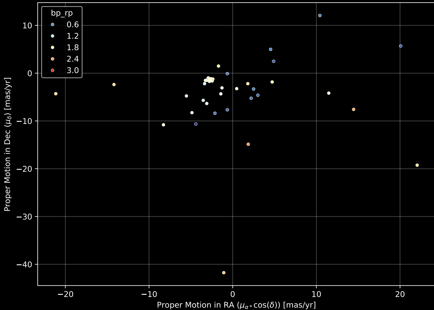
APOGEE DR17 Field: [SGRC-3] Proper Motion Diagram (n= 145)
