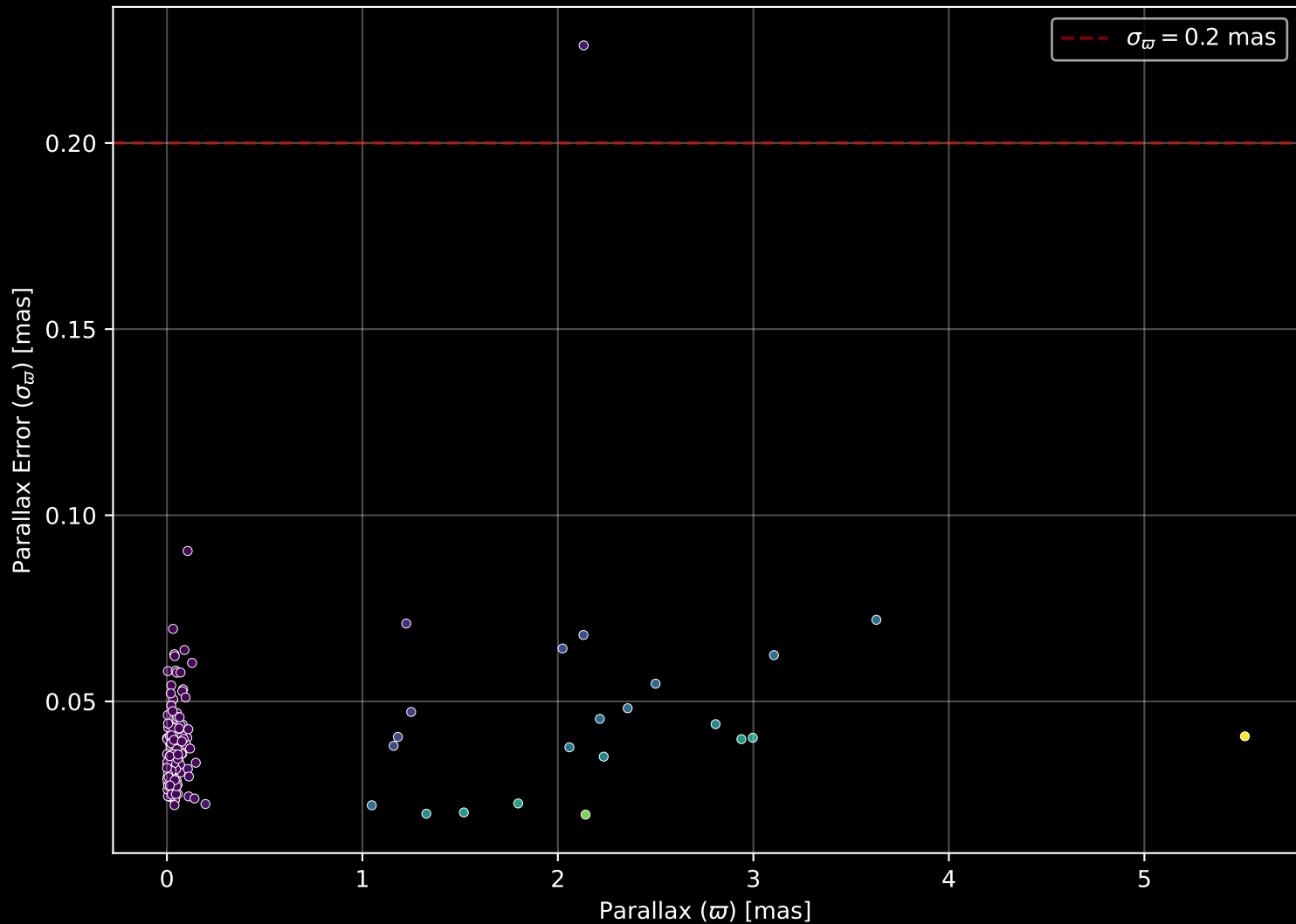
APOGEE DR17 Field: [SGRC-3] Parallax Quality (n= 145)
